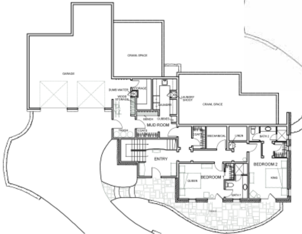
LOWER LEVEL FLOOR PLAN (1,216 SQ. FT.)
